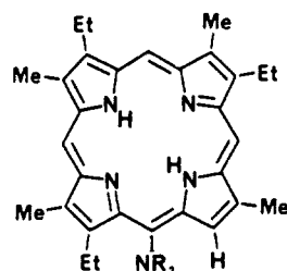
19 R = Me
